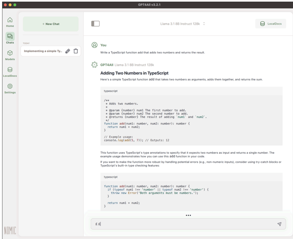
Figure 9.1 User Interface of GPT4All
