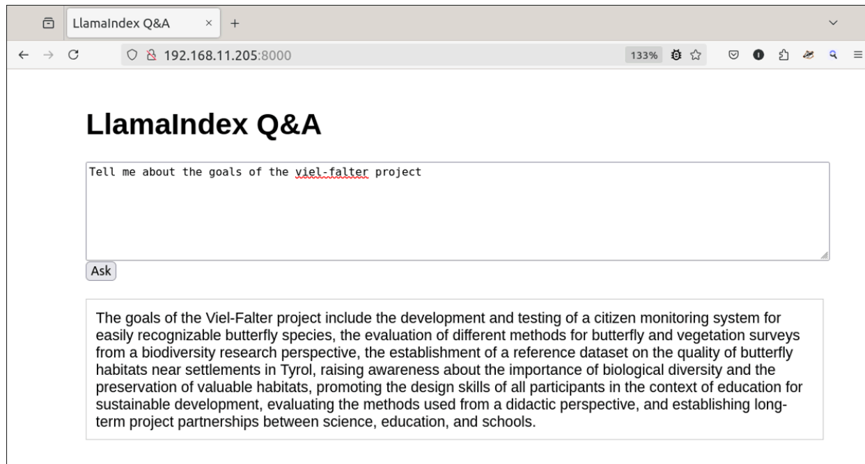
Figure 12.1 Our Quick Introduction to RAG
